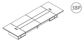
66P6006 6000Wx2000Dx750H (12067)
