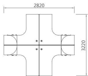
18L2024 屏风位 2820Wx3220Dx1200H (10107)
