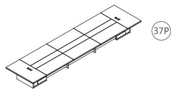
66P6006+66P2006YS 8000Wx2000Dx750H
