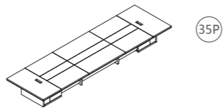
66P5006+66P2006YS 7000Wx2000Dx750H
