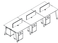
09B2404+09B1204YS 3600Wx1200Dx750H (7000)
