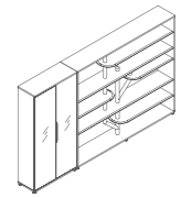
09F3301 3300Wx400Dx2000H (9000)
