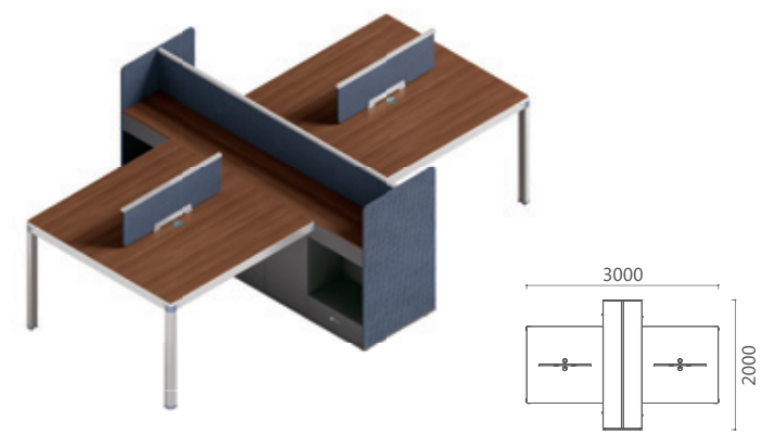
08B3004 职员桌 3000Wx2000Dx1050H (4883)
