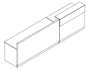
09R3201 3200Wx670Dx1000H (4133) 09R2601 2600Wx670Dx1000H (4000)
