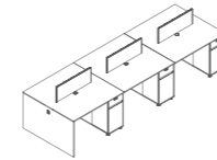
09B2409+09B1209YS 3600Wx1200Dx750H (4700)
