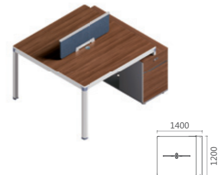
08B1402 职员桌 1400Wx1200Dx750H (2250)
