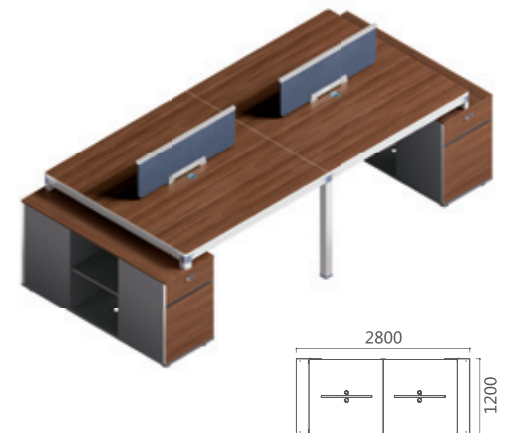
08B2802 职员桌 2800Wx1200Dx750H (3983)
